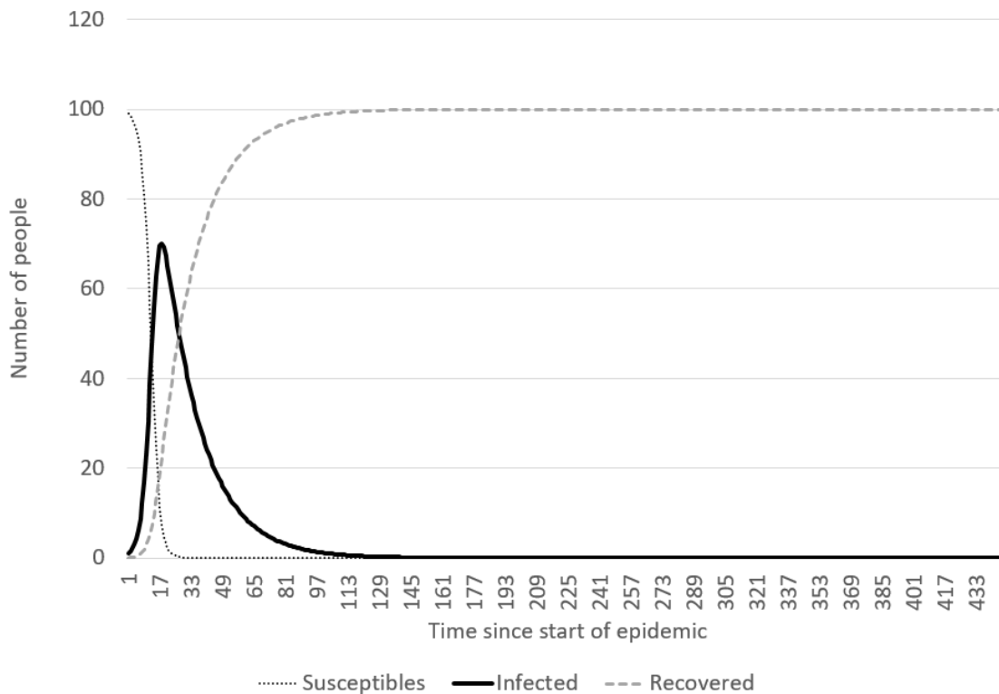
Figure 2. Solution to Kermack-McKendrick SIR model for N=100 , I=1 , c=.005 , r=.05 .
